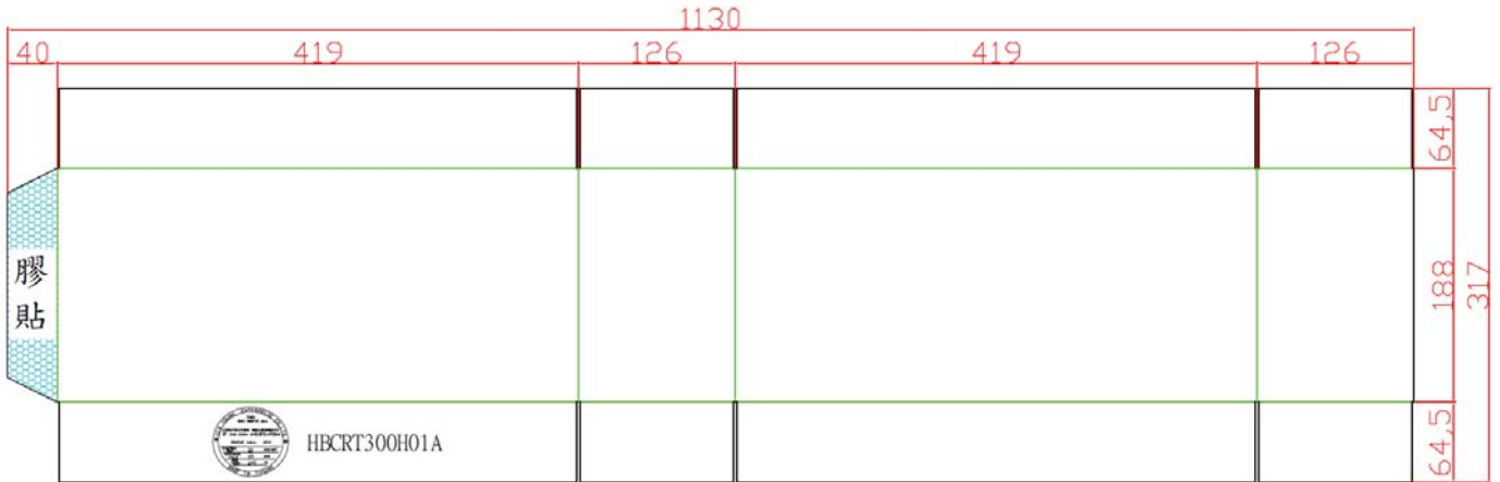
KT300HA carton size
