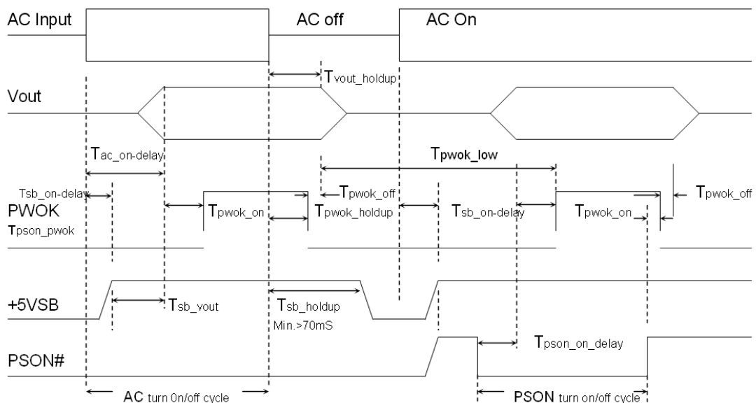
Figure 2: Turn On/Off Timing
