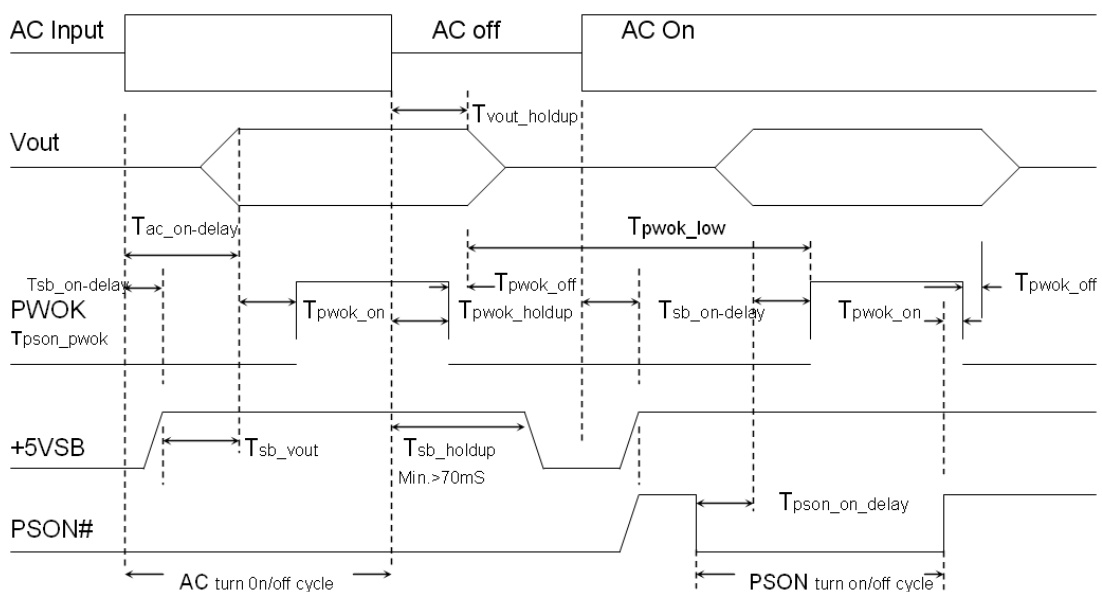
Figure 2: Turn On/Off Timing
